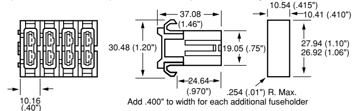
Typical Multiple Mounting (Fuseholders interlocked)
